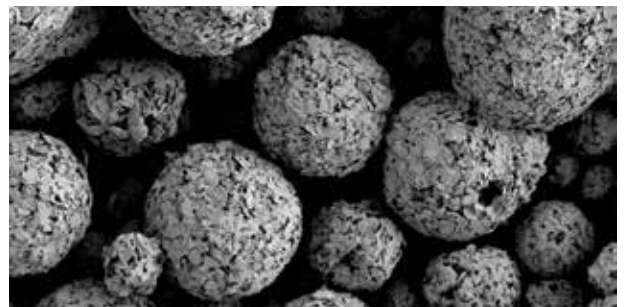
SEM micrograph: Grade CFP 012P
