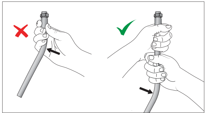
Proper Bend Location
