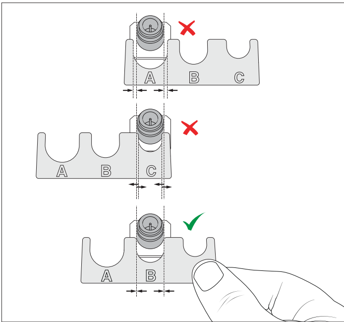
Closure Gauge Use
