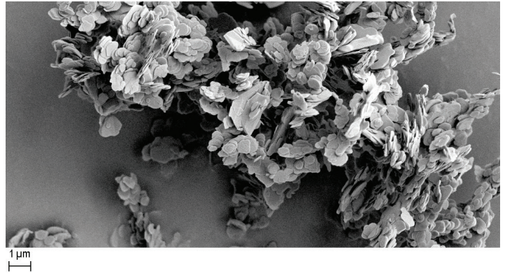
SEM micrograph: Grade CFP 003SF
