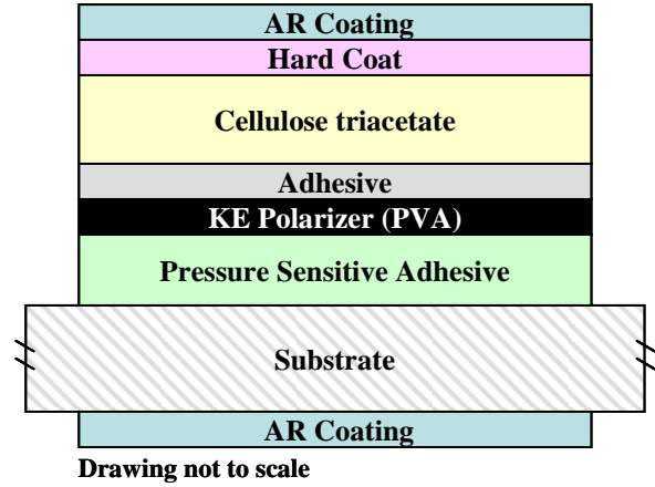
Fig. 5. Typical KE polarizer based projection component.
