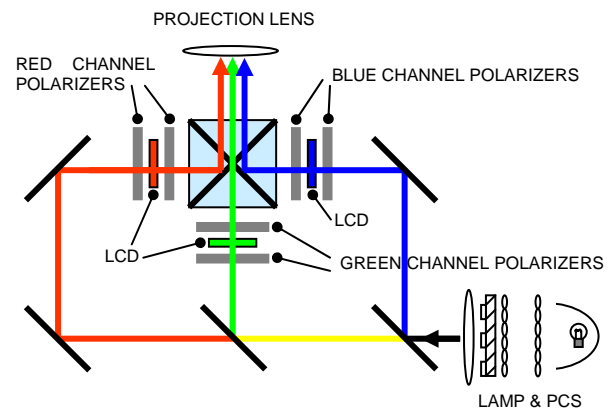
Fig. 2. Diagram of a typical HTPS light engine.
