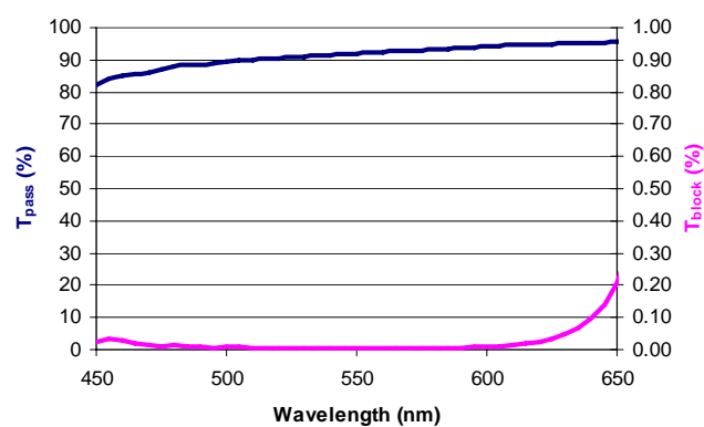
Fig. 3. Typical KE T_{\text{pass}} and T_{\text{block}} performance by wavelength (with anti-reflection coating).
