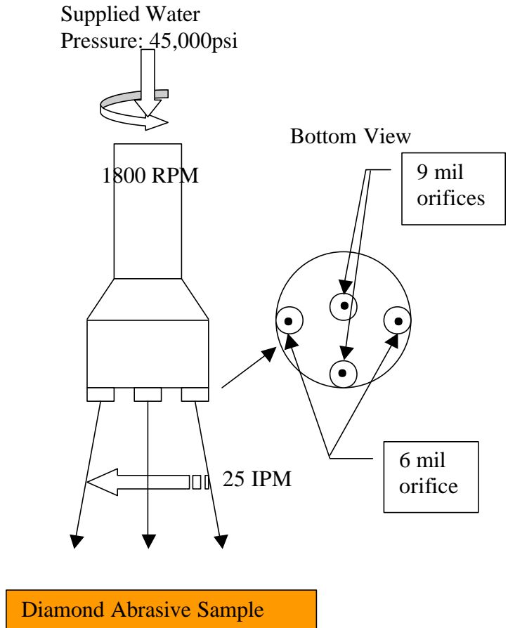
Fig. 1 Washing Apparatus Schematic
