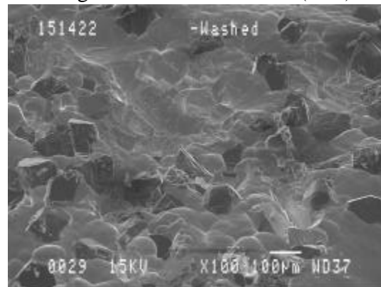
Fig. 13 Vendor B Washed (100X)
