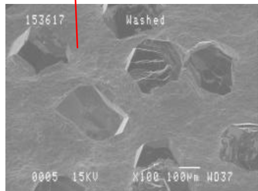
Fig. 9 3M Std. Washed (100X)
