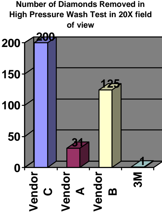
Figure 15. Diamond loss comparison for various diamond pad conditioners
