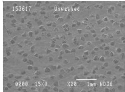
Fig. 6 3M Std. Unwashed (20X)
