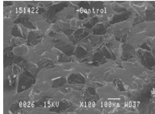
Fig. 11 Vendor B Unwashed (100X)
