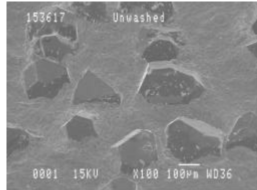
Fig. 7 3M Std. Unwashed (100X)
