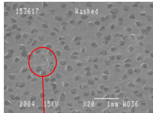
Fig. 8 3M Std. Washed (20X)
