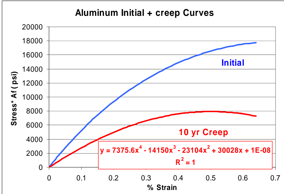
Figure 18. Aluminum initial and 10-year stress-strain curves
