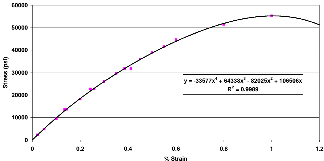
Figure 6. Fourth order polynomial fit to Conductor Stress-strain behavior
