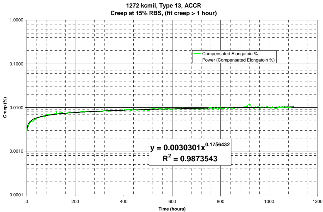
Figure 1. Creep strain vs. time for 1272-kcmil conductor at 15% RBS load
