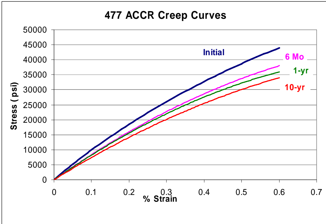
Figure 12. Creep Stress-Strain Curves for 477-kcmil, 3M™ Composite Conductor
