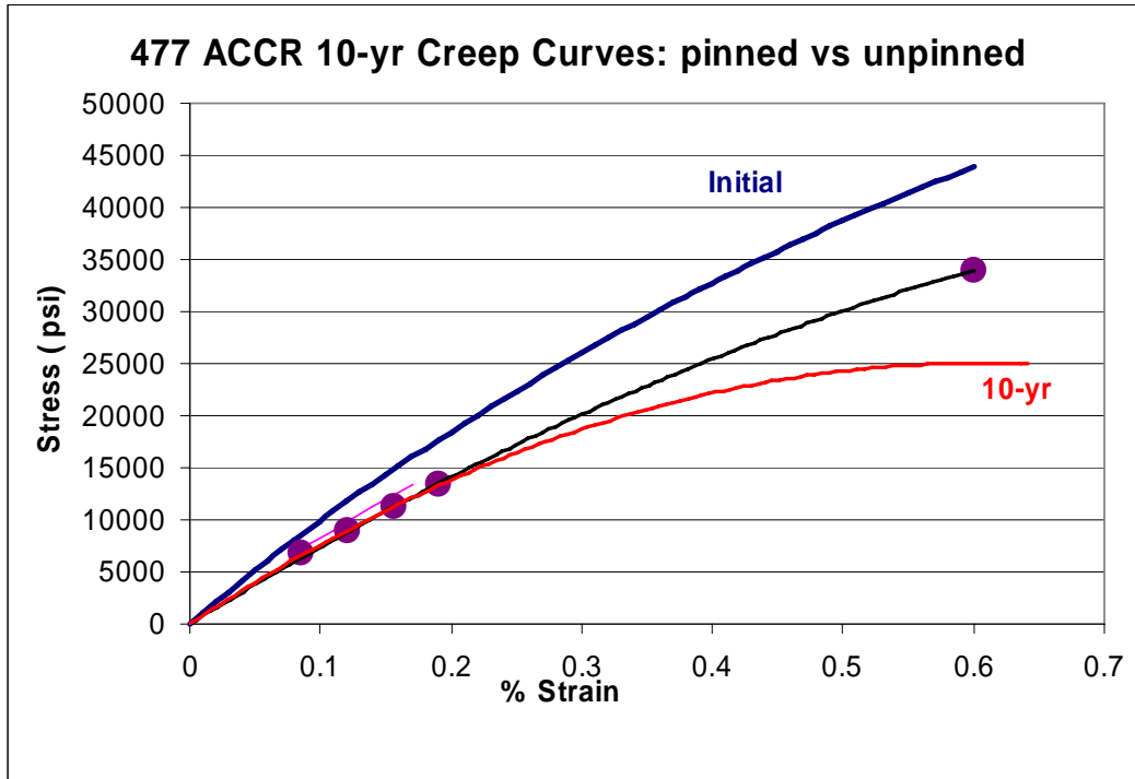
Figure 11. 10-year creep curves for 477-kcmil, 3M™ Composite Conductor with and without the artificial point at 0.6% strain
