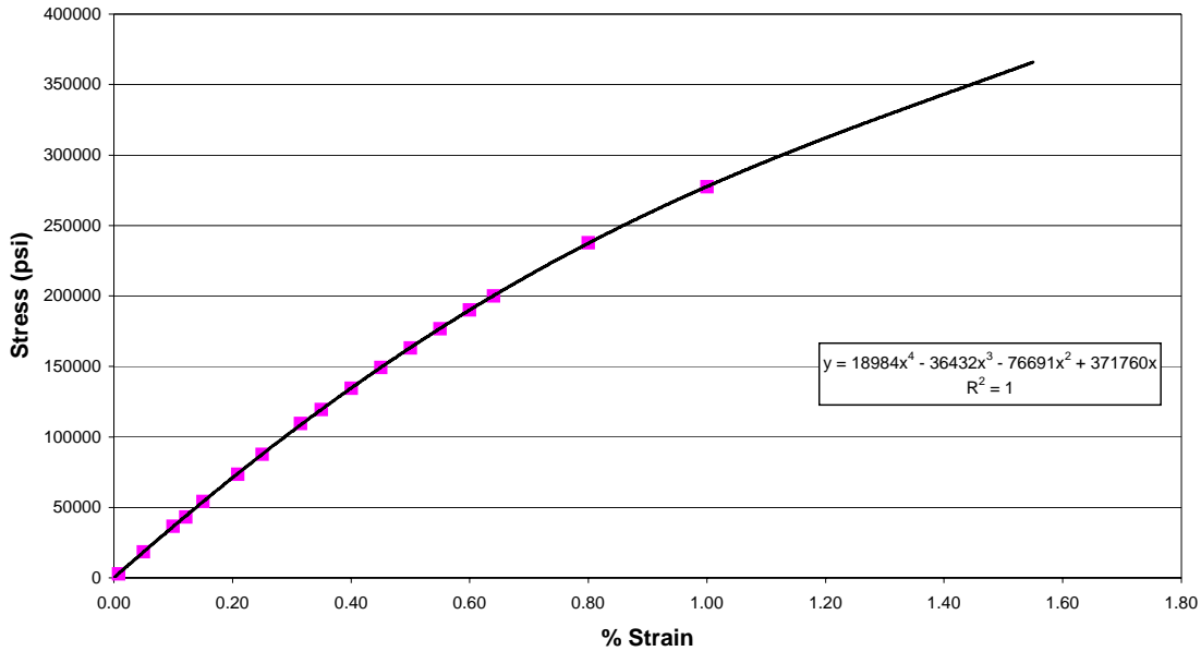
Figure 7. Fourth-order polynomial fit for 1272 ACCR core.
