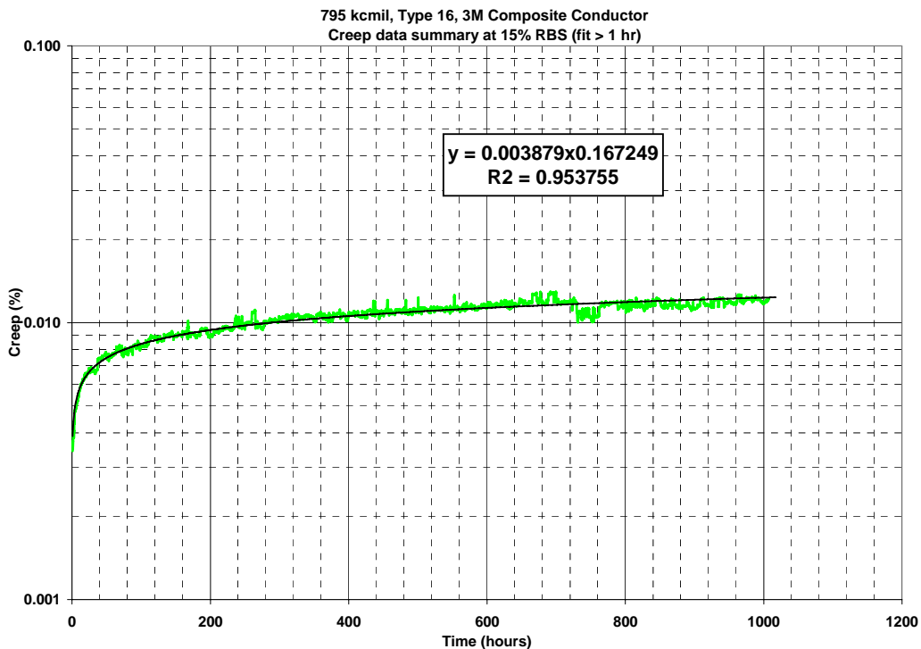
Figure 1. Creep strain vs. time for 795-kcmil, 3M™ Composite Conductor at 15% RBS
