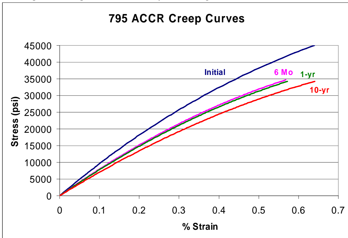
Figure 12. Creep Stress-Strain Curves for 795-kcmil, 3M™ Composite Conductor
