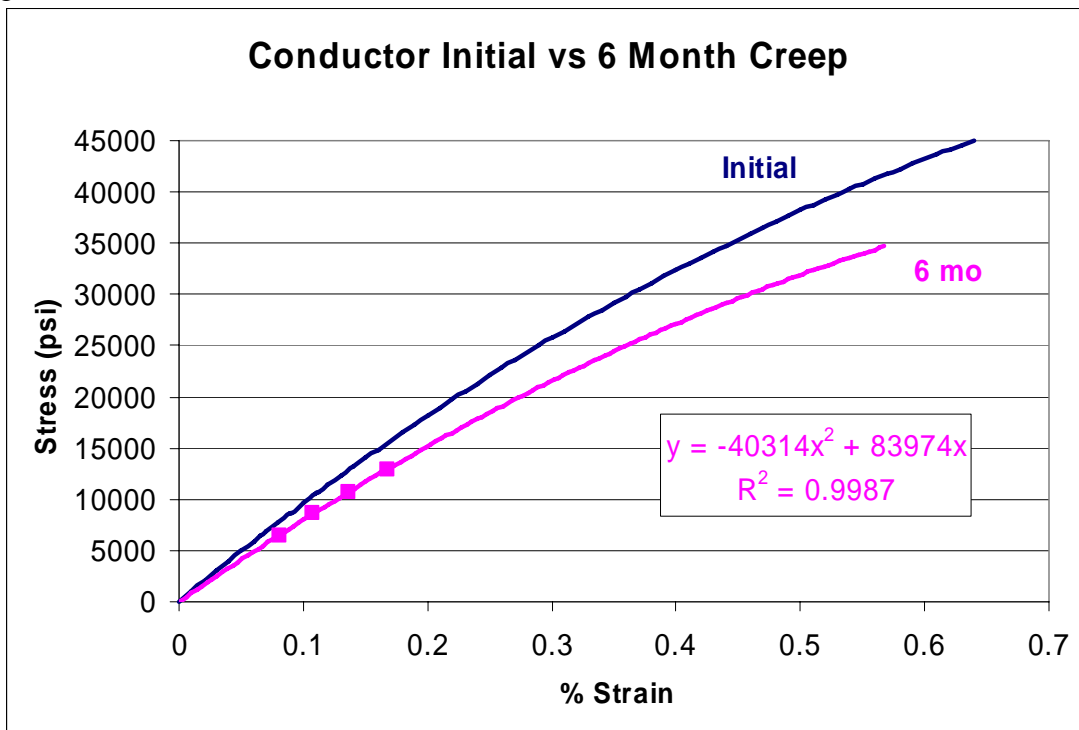
Figure 11. Six-month creep curve for 795-kcmil, 3M™ Composite Conductor
