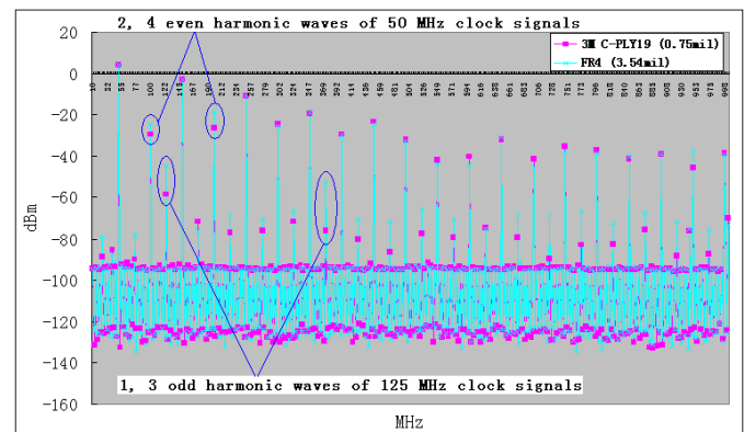
Fig. 15. Comparison of the 50 MHz clock signal frequency spectrums between the embedded capacitance and the conventional FR-4 material boards
