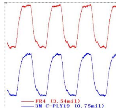
Fig. 14. Comparison of the 50 MHz clock signal measured wave between the embedded capacitance and the conventional FR-4 material boards
