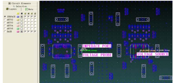
Fig. 5. Simulation setup of the embedded capacitance material board and the conventional FR-4 material board
