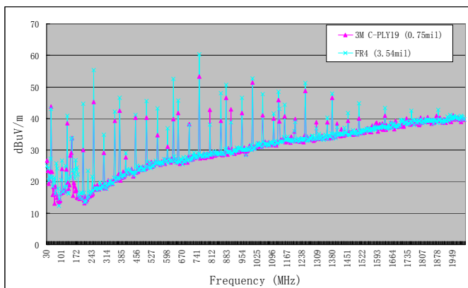
Fig.11. Comparison of the RE testing results of the embedded capacitance and the conventional FR-4 material boards
