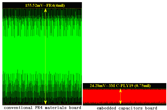
Fig. 9. Comparison of the power ripple noise of the embedded capacitance and the conventional FR-4 material boards
