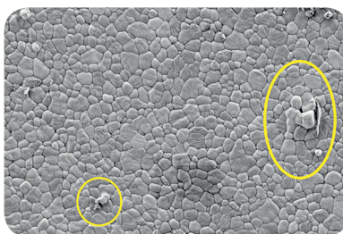
Generic zirconia – highlighted in purity and pore
