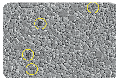
Branded competitive zirconia – highlighted segregated Alumina grains
